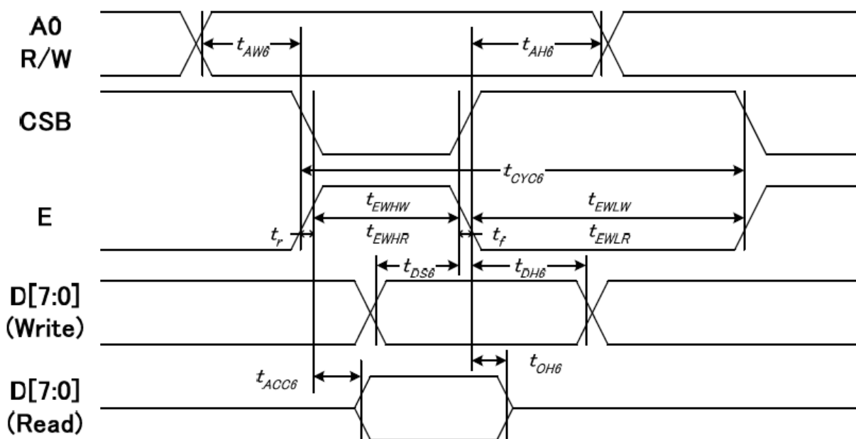
图 6. 从 CPU 写到 ST7586S (Writing Data from CPU to ST7586S)
