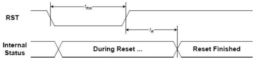
FIGURE 20: Reset Characteristics
