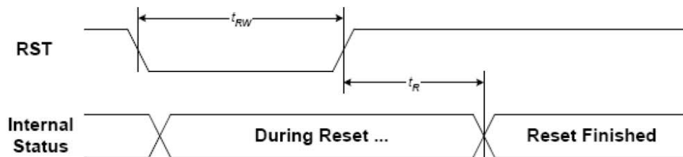
FIGURE 20: Reset Characteristics
