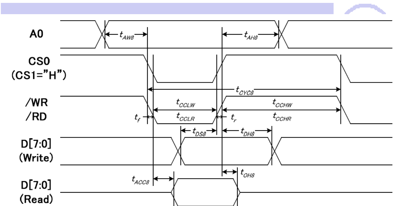
图 4. 从 CPU 写到 ST7525I (Writing Data from CPU to ST7525I)
